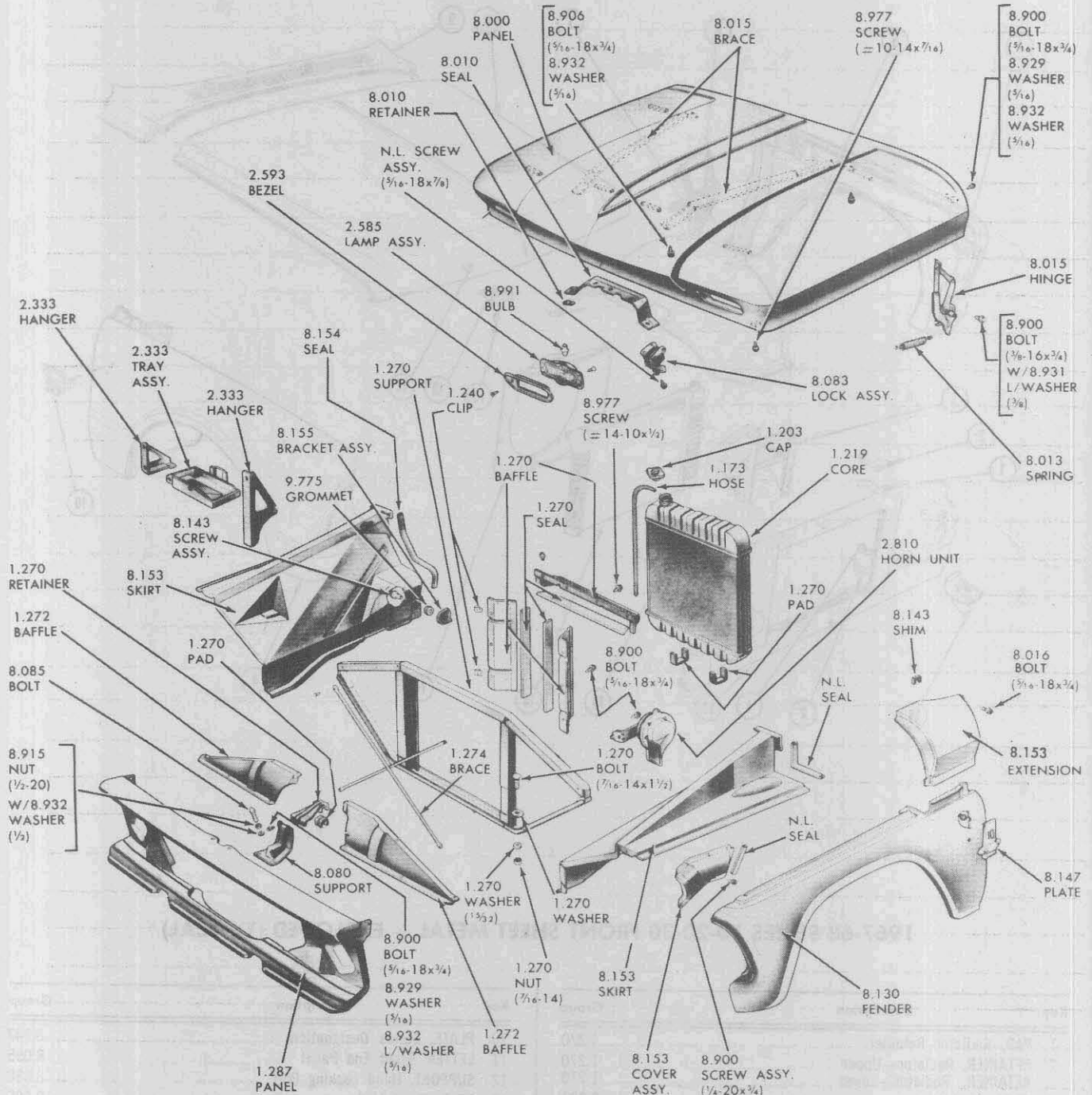
1965-66 FRONT END SHEET METAL — TYPICAL
