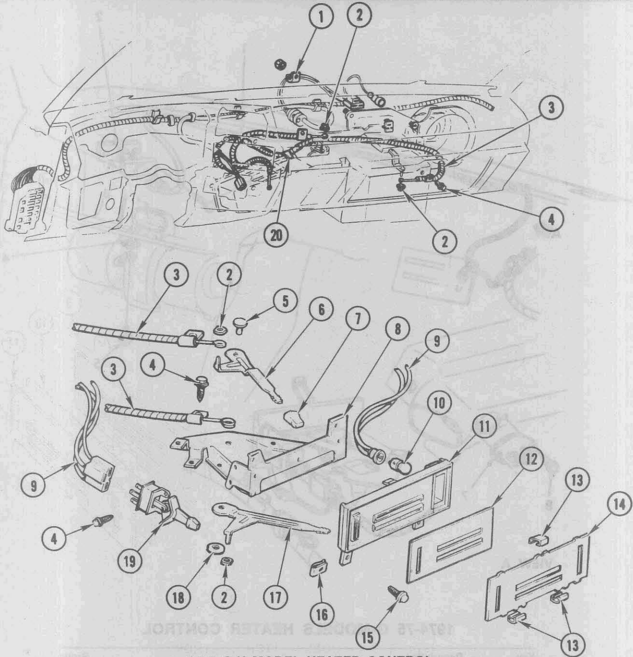
1973 C-K MODEL HEATER CONTROL
